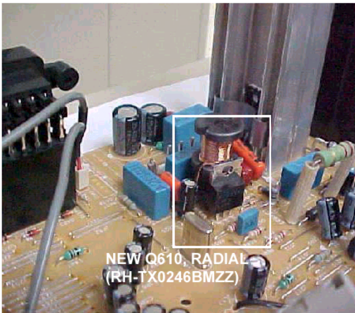
Figure 2: Mother Unit F7315BMN6, Component Side.
